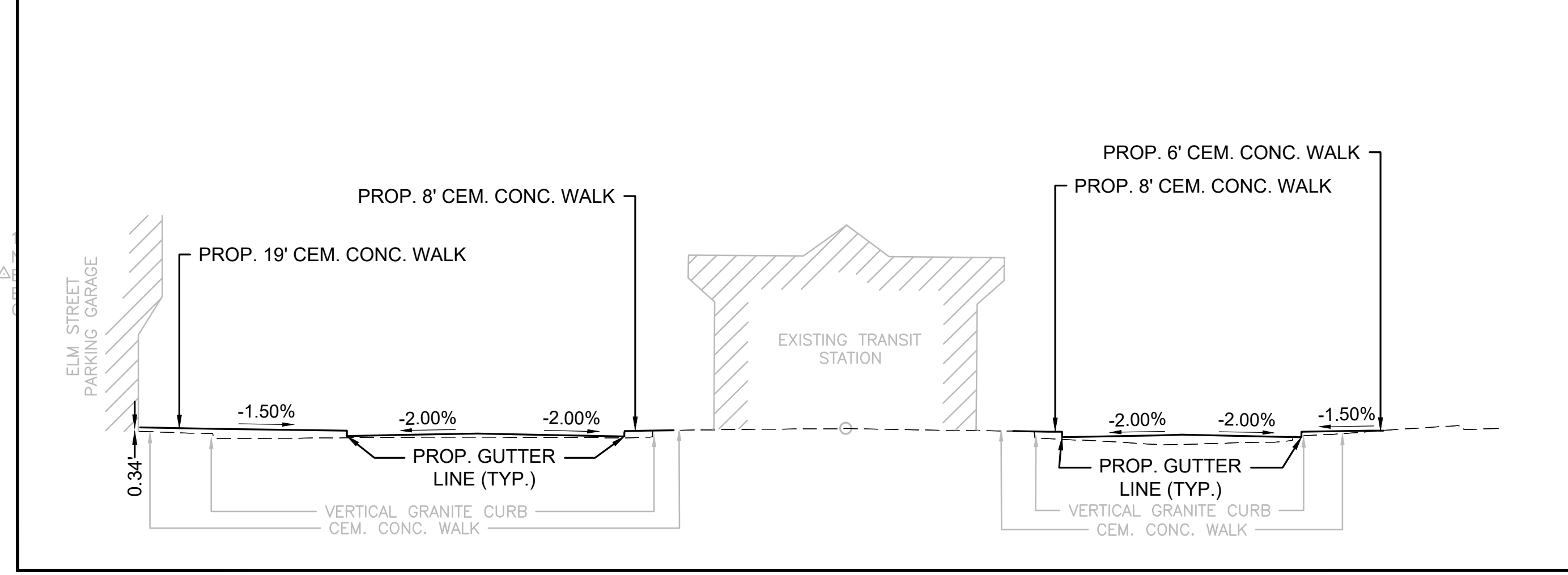
PEDESTRIAN PLAZA HYBRID SECTION A-A 0 10 20 30 40 SCALE: 1" = 10'
